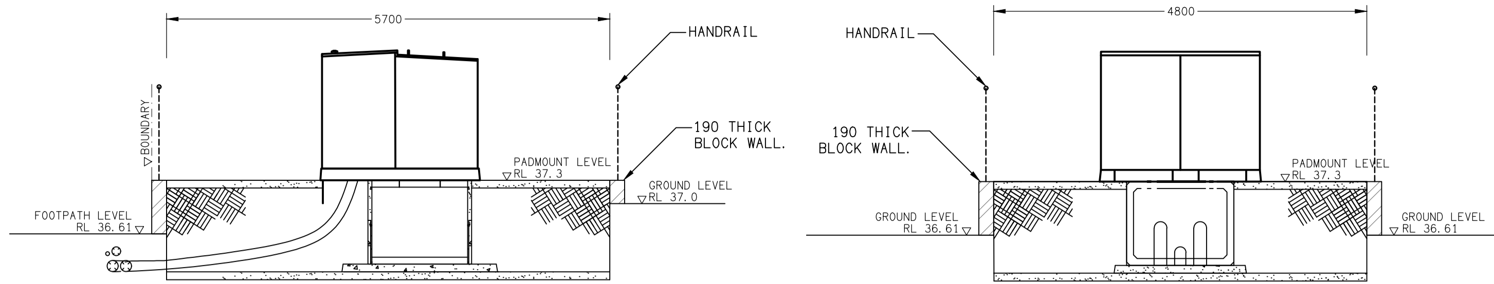
DETAIL A PADMOUNT SECTION VIEW SCALE 1:50
