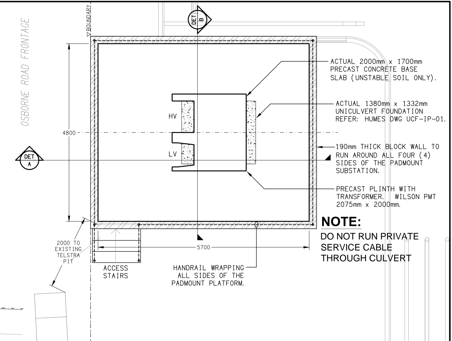
DETAIL PLAN ENERGEX POSITIONING OF PADMOUNT ON UNICULVERT SCALE 1:50
